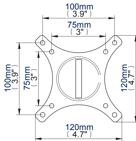
Interface Plate
